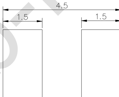
RECOMMENDED SOLDERING PAD DESIGN
